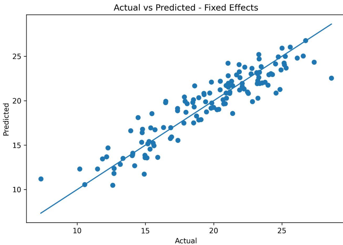
Figure 10.3: Actual vs Predicted Values for Fixed Effects Model
